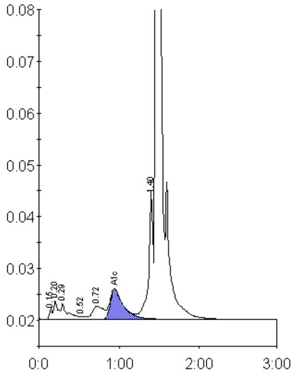
Peak table - ID: CA011566
